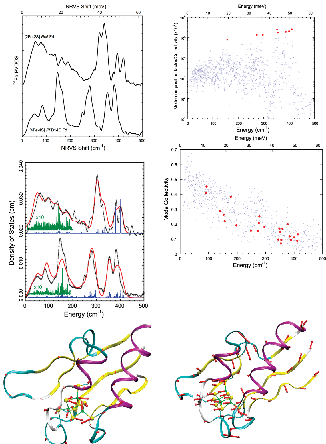
Figure 5. Full protein calculation analysis of oxidized PfD14C Fd . Experimental PVDOS (black lines) of oxidized Rc6 Fd and oxidized PfD14C Fd (top left). Experimental PVDOS (black lines) vs calculated spectra (red lines) for reduced Rc6 Fd and oxidized PfD14C Fd (middle left). Sticks represent the mode composition factors of individual modes. Degree of collectivity for normal modes with largest mode composition factors highlighted in red (bottom) and mode composition factor divided by the degree of collectivity to emphasize cluster-centered normal modes (top) (two top right panels). The bottom panels are illustrations of calculated normal modes at (left) 157\text{ cm}^{-1} and (right) 16\text{ cm}^{-1} .
