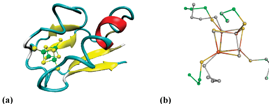
Chart 1. (a) VMD 17 Cartoon Representation of the [Fe 4 S 4 ] 2+ Form of Oxidized PfD14C Ferredoxin (PDB entry 2Z8Q) and (b) Close-Up of the Crystallographically Observed Cluster Site (color) Compared to a Hypothetical Fe 4 S 4 (SCCC) 4 Model with C 2 Symmetry (gray)
