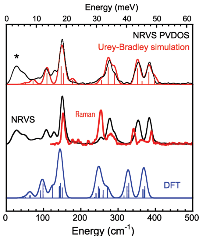
Figure 1. Data and simulations for (\text{Ph}_4\text{P})_2[^{57}\text{Fe}_4\text{S}_4\text{Cl}_4] . From top to bottom: experimental ^{57}\text{Fe} PVDOS (black line) and Urey–Bradley simulation (red line), experimental ^{57}\text{Fe} PVDOS (black line) compared with the resonance Raman spectrum (red line), and DFT calculations for [\text{Fe}_4\text{S}_4\text{Cl}_4]^{2-} (blue line). The asterisk indicates the low-frequency region of acoustic modes not included in the calculations. Sticks show frequencies and relative intensities of calculated normal modes before linewidth broadening.
