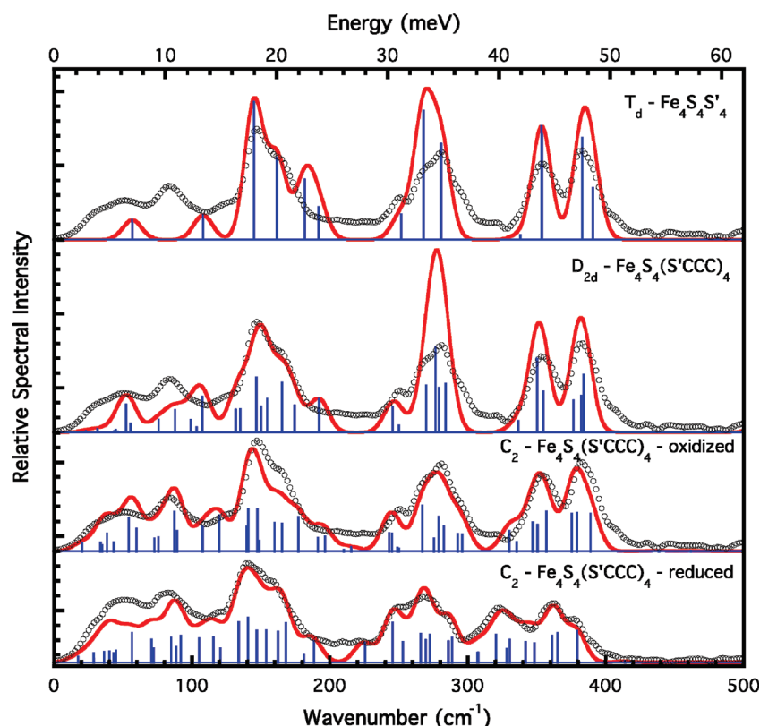
Figure 3. Urey–Bradley force field simulations (red lines) vs experimental Pf D14C PVDOS (O). From top to bottom: oxidized protein vs the \text{Fe}_4\text{S}_4(\text{S}')_4 model in T_d symmetry, the \text{Fe}_4\text{S}_4(\text{S}'\text{CCC})_4 model in D_{2d} symmetry, the \text{Fe}_4\text{S}_4(\text{S}'\text{CCC})_4 model in C_2 symmetry, and (d) the reduced protein vs \text{Fe}_4\text{S}_4(\text{S}'\text{CCC})_4 model in C_2 symmetry. Sticks correspond to individual normal-mode frequencies and relative intensities before broadening.
